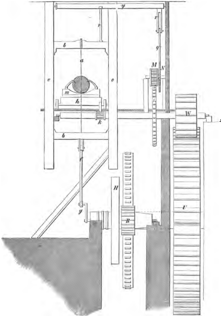
Fig. 296.—Forest sawmill driven by water-power.
